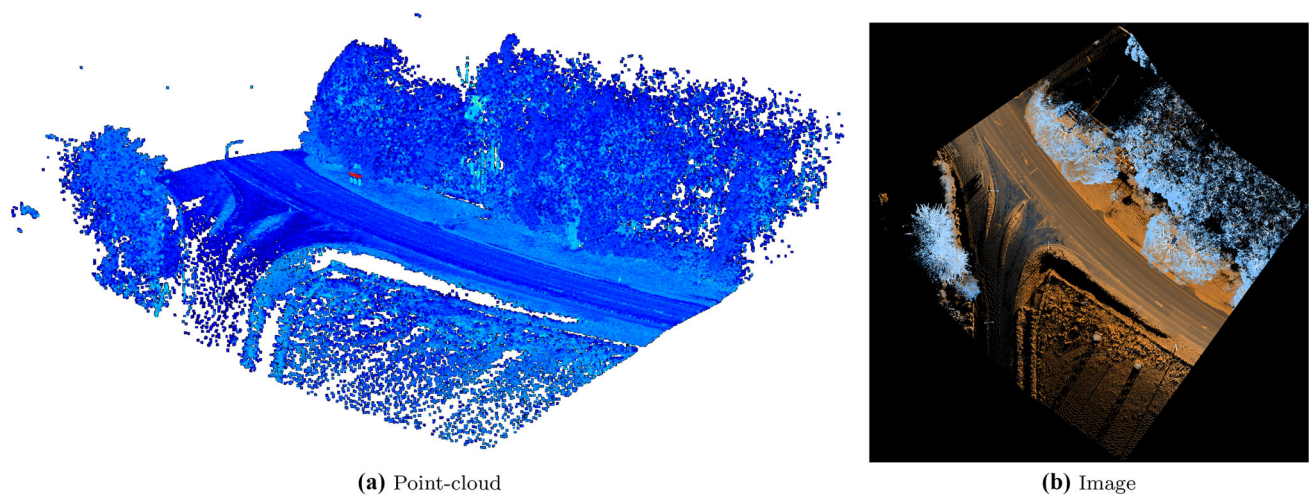
Fig. 2 Road environment can clearly be seen in the point-cloud data. The image has intensity in the red colour channel, height in the blue colour channel and an average of the two in the green colour channel
