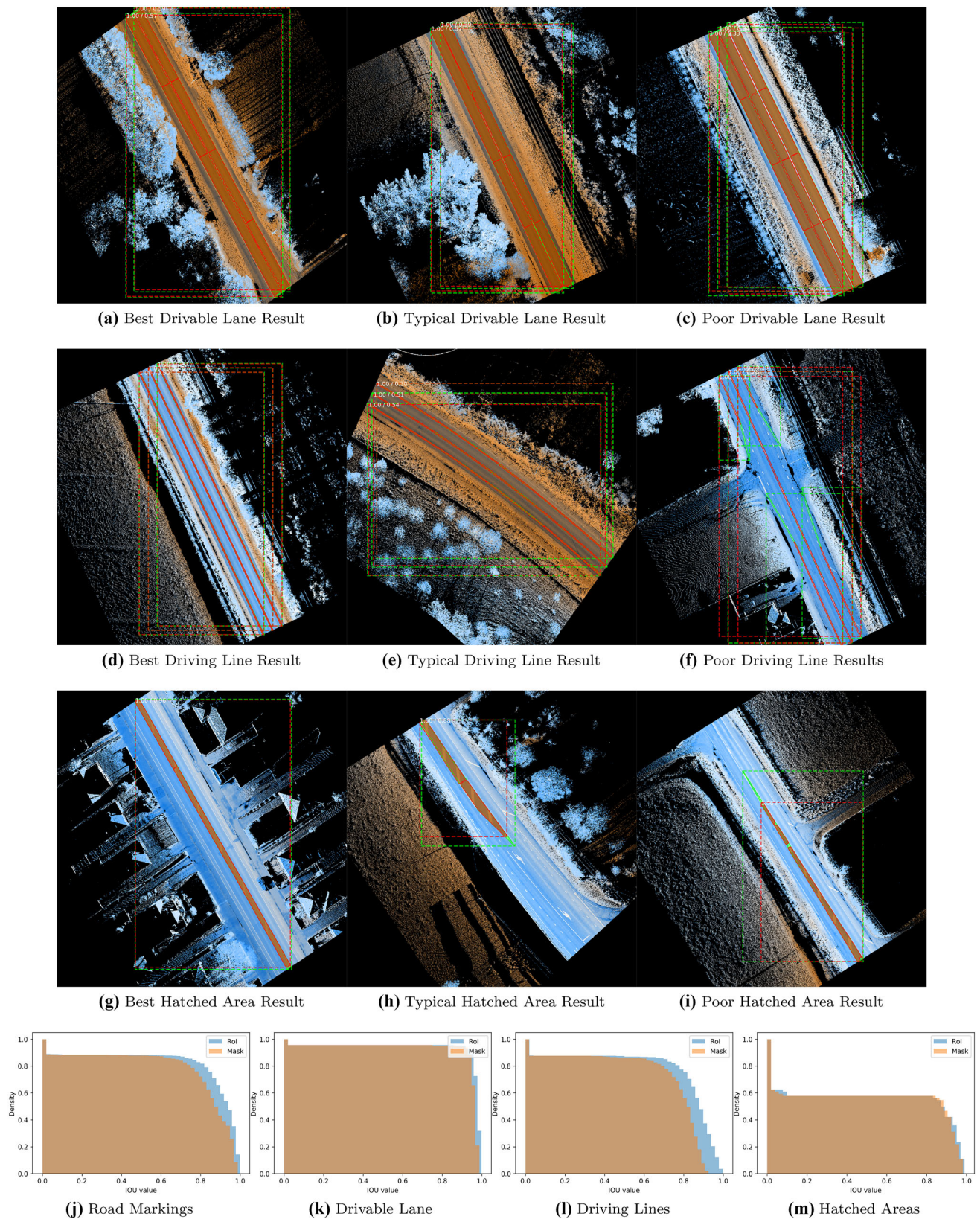
Fig. 10 Road marking segmentation results. In (a–i) the green and red represent the ground truth and predicted mask respectively. j–m are reverse cumulative IoU distributions
