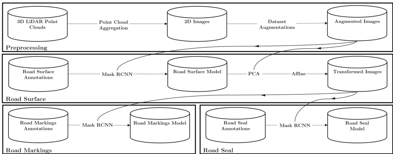
Fig. 4 Proposed framework
