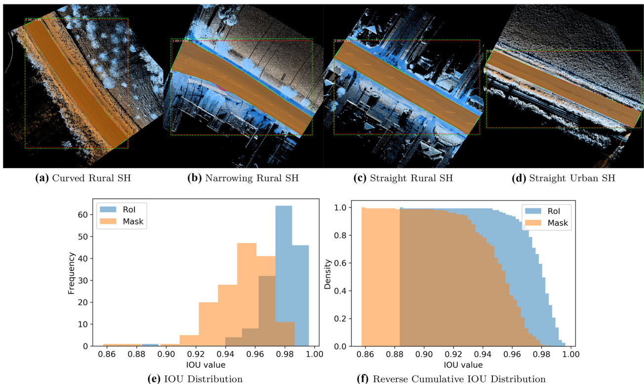
Fig. 11 Road seal test results: a–d examples of predicted masks for road surface instances compared to ground truth masks, e–f test IoU scores for RoIs and masks
